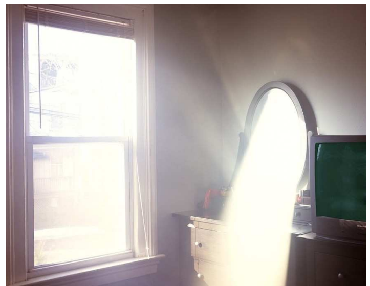
Visible light, Alexander HARDING
